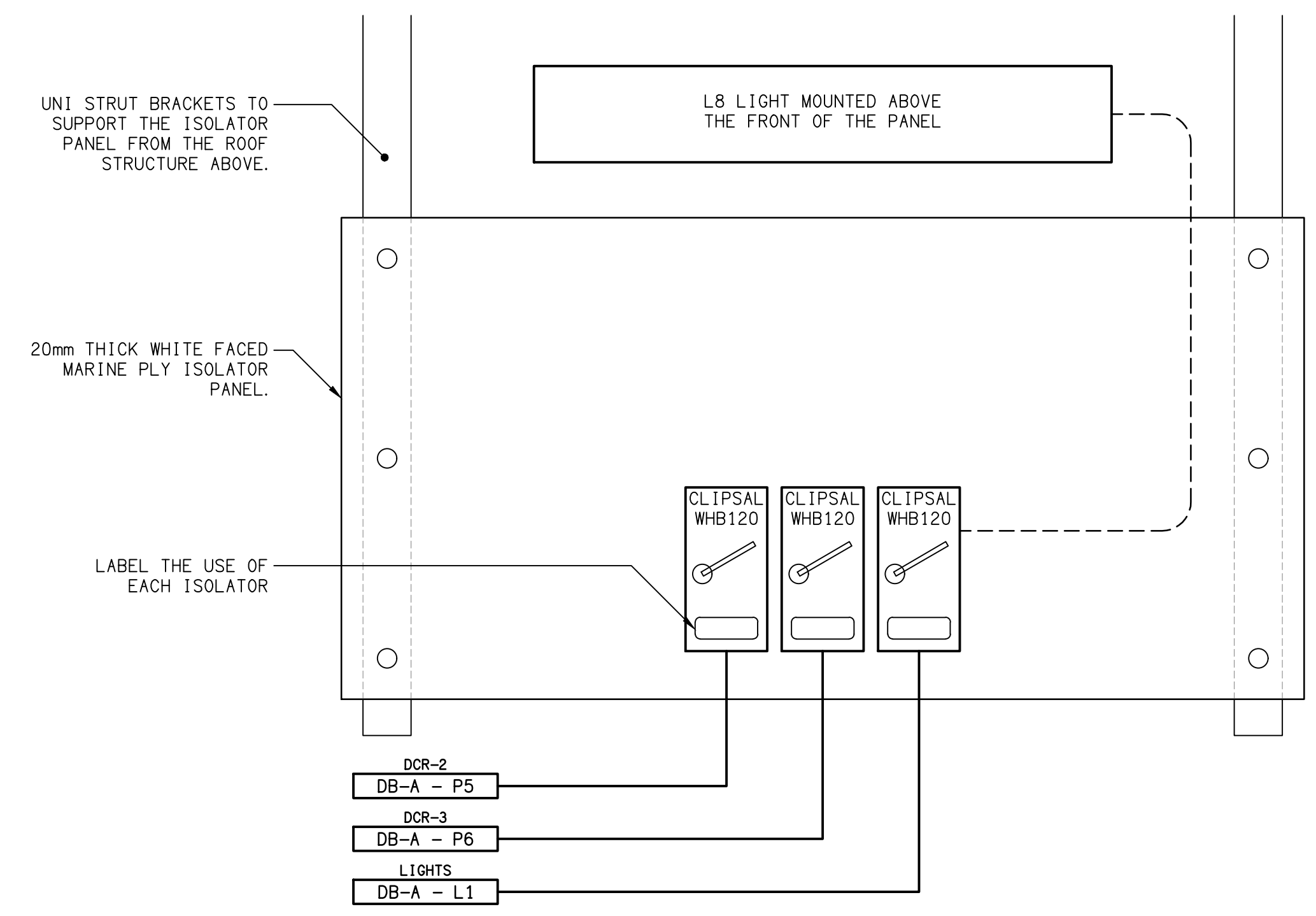
DETAILS ISOLATOR PANEL ELEVATIONS NOT TO SCALE
